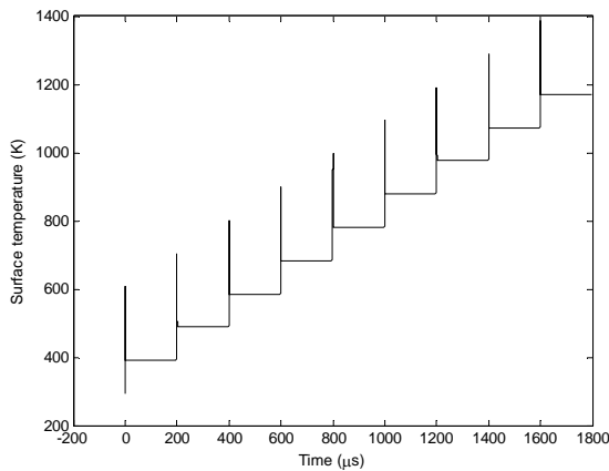
Fig. 2. Particle surface temperature versus time for multiple laser pulses ( J = 1688 \text{ J/m}^2 , t_p = 75 \text{ ns} , r_0 = 11 \text{ }\mu\text{m} , T_i = 293 \text{ K} , p = 700 \text{ kPa} , f = 5000 \text{ Hz} ).
