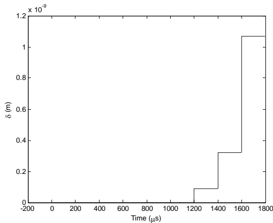
Fig. 3. Thickness of deposited film versus time for multiple laser pulses ( J = 1688 \text{ J/m}^2 , t_p = 75 \text{ ns} , r_0 = 11 \text{ }\mu\text{m} , T_i = 293 \text{ K} , p = 700 \text{ kPa} , f = 5000 \text{ Hz} ).
