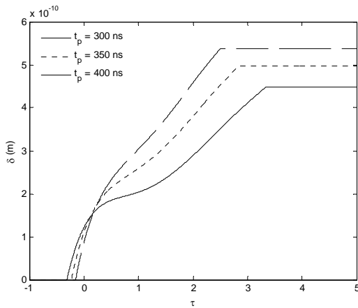
Fig. 6. Thickness of deposited film during the first laser pulse for various values of laser pulse width ( J = 13 \text{ kJ/m}^2 , r_0 = 11 \text{ }\mu\text{m} , T_i = 293 \text{ K} , p = 700 \text{ kPa} , f = 5000 \text{ Hz} ).
