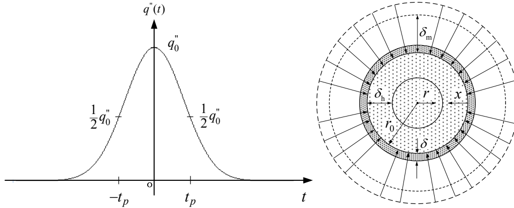
Fig. 1. The physical model.
