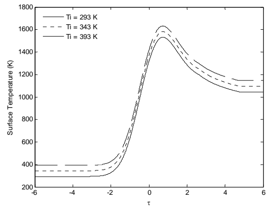
Fig. 7. Surface temperature during the first laser pulse for various values of particle initial temperature ( J = 13 \text{ kJ/m}^2 , t_p = 350 \text{ ns} , r_0 = 11 \text{ }\mu\text{m} , p = 700 \text{ kPa} , f = 5000 \text{ Hz} ).
