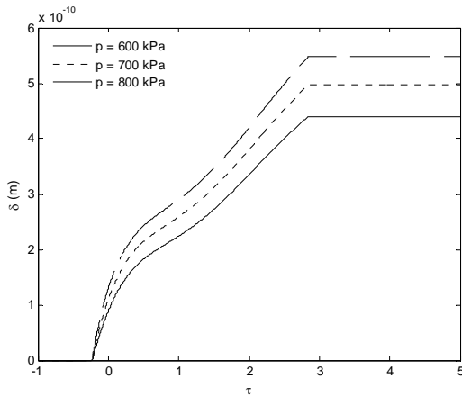
Fig. 13. Thickness of deposited film during the first laser pulse for various values of total pressure in the reaction chamber ( J = 13 \text{ kJ/m}^2 , t_p = 350 \text{ ns} , r_0 = 11 \text{ }\mu\text{m} , T_i = 293 \text{ K} , f = 5000 \text{ Hz} ).
