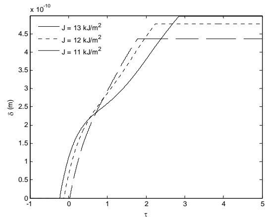
Fig. 12. Thickness of deposited film during the first laser pulse for various values of laser fluence ( t_p = 350 \text{ ns} , r_0 = 11 \mu\text{m} , T_i = 293 \text{ K} , p = 700 \text{ kPa} , f = 5000 \text{ Hz} ).
