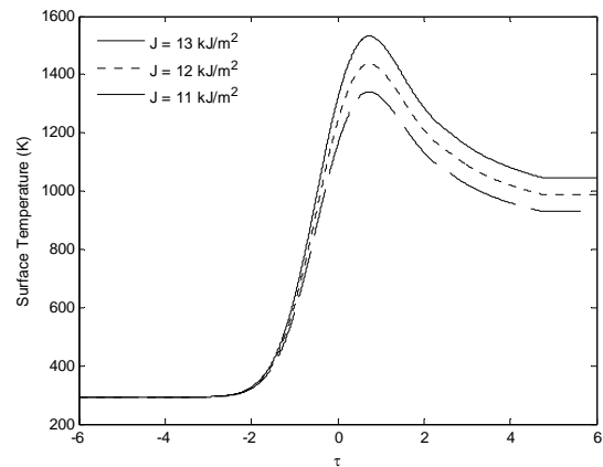
Fig. 11. Surface temperature during the first laser pulse for various values of laser fluence ( t_p = 350 \text{ ns} , r_0 = 11 \mu\text{m} , T_i = 293 \text{ K} , p = 700 \text{ kPa} , f = 5000 \text{ Hz} ).
