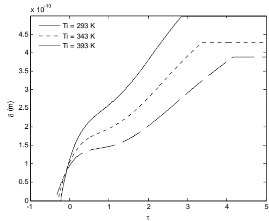
Fig. 8. Thickness of deposited film during the first laser pulse for various values of particle initial temperature ( J = 13 \text{ kJ/m}^2 , t_p = 350 \text{ ns} , r_0 = 11 \text{ }\mu\text{m} , p = 700 \text{ kPa} , f = 5000 \text{ Hz} ).
