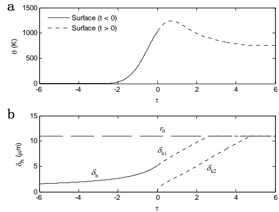
Fig. 4. Surface temperature and thermal penetration depth during the first laser pulse ( J = 13 \text{ kJ/m}^2 , t_p = 350 \text{ ns} , r_0 = 11 \text{ }\mu\text{m} , T_i = 293 \text{ K} , p = 700 \text{ kPa} , f = 5000 \text{ Hz} ). (a) Temperatures. (b) Thermal penetration depth.
