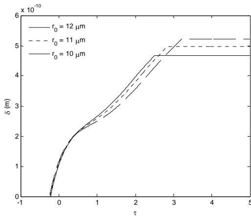
Fig. 10. Thickness of deposited film during the first laser pulse for various values of particle radius ( J = 13 \text{ kJ/m}^2 , t_p = 350 \text{ ns} , T_i = 293 \text{ K} , p = 700 \text{ kPa} , f = 5000 \text{ Hz} ).
