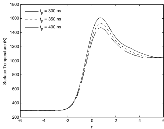
Fig. 5. Surface temperature during the first laser pulse for various values of laser pulse width ( J = 13 \text{ kJ/m}^2 , r_0 = 11 \text{ }\mu\text{m} , T_i = 293 \text{ K} , p = 700 \text{ kPa} , f = 5000 \text{ Hz} ).
