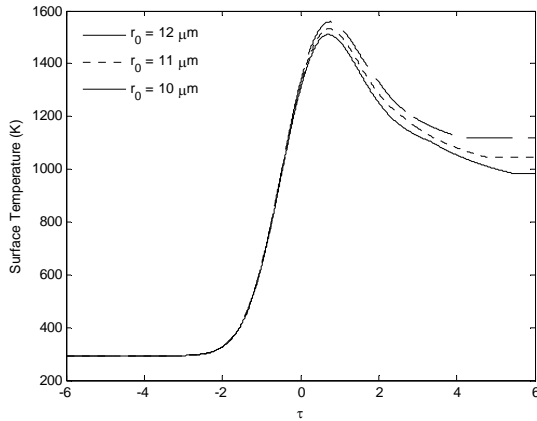
Fig. 9. Surface temperature during the first laser pulse for various values of particle radius ( J = 13 \text{ kJ/m}^2 , t_p = 350 \text{ ns} , T_i = 293 \text{ K} , p = 700 \text{ kPa} , f = 5000 \text{ Hz} ).
