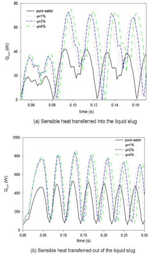
Fig. 2 Effect of nanofluid on sensible heat transferred into the liquid slug for d_p=38.4nm
