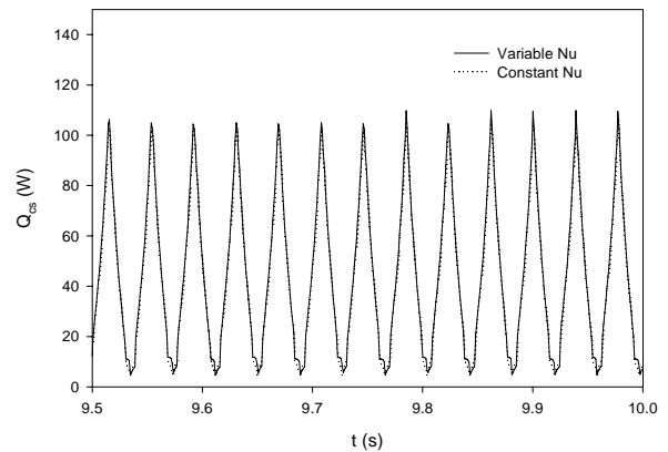
(b) Sensible heat transferred out from the liquid slug
